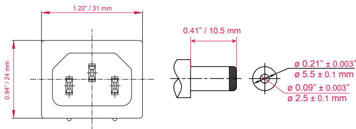
INPUT IEC320 C14 AC PIN 100 ~ 240 VAC
