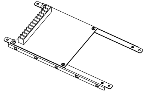
PRE-ASSEMBLED GEMC-BM BURG MODULE
