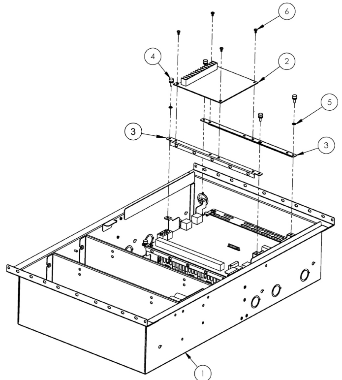
EXPLODED VIEW OF GEMC-BM BURG MODULE. SEE TABLE BELOW FOR NUMBER DESCRIPTIONS
