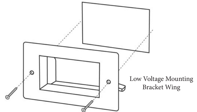
Installation Diagram - Front View
